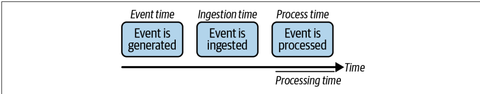
Figure 5-6. Event, ingestion, process, and processing time
