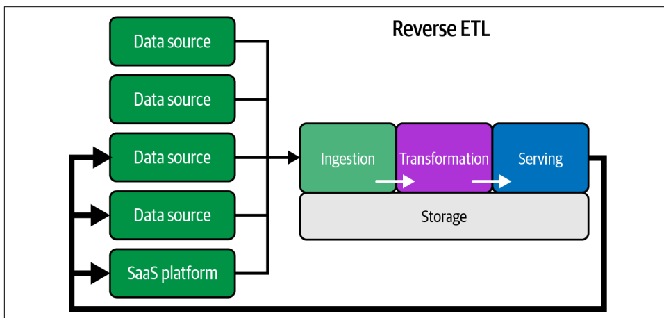
Figure 9-5. Reverse ETL
